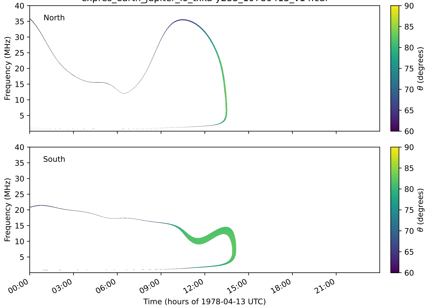
expres_earth_jupiter_io_txka-y235_19780413_v14.cdf
