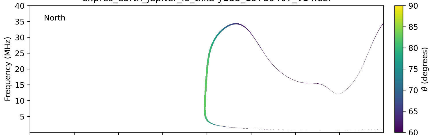
expres_earth_jupiter_io_txka-y235_19780407_v14.cdf
