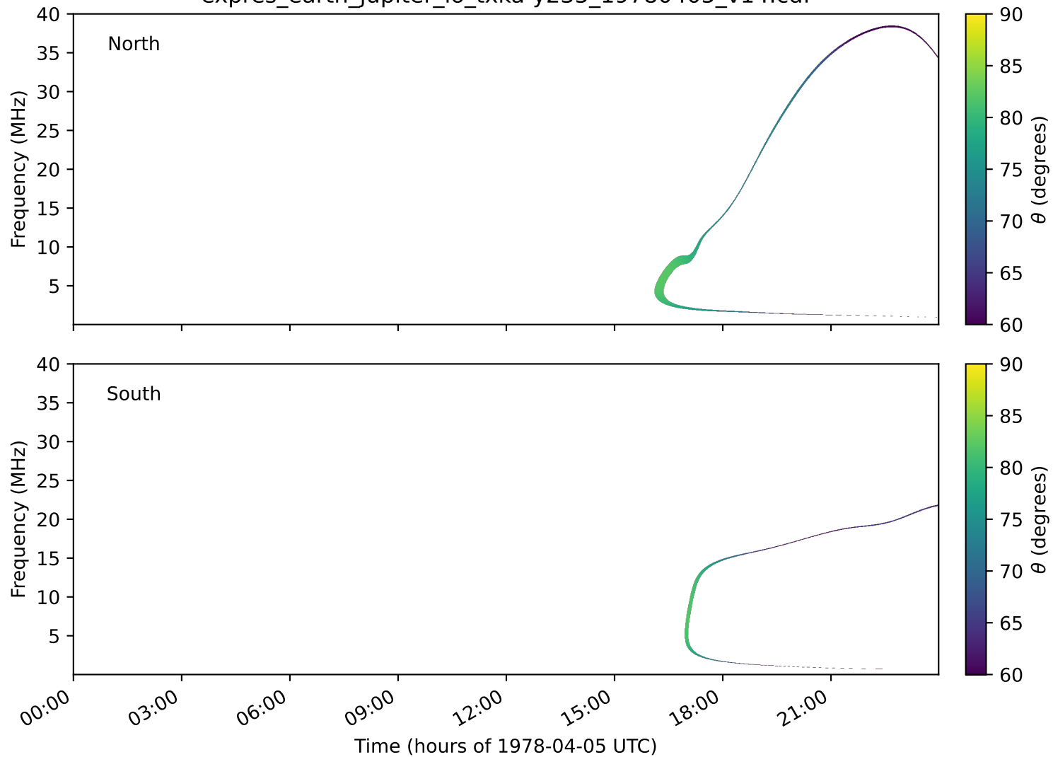
expres_earth_jupiter_io_txka-y235_19780405_v14.cdf
