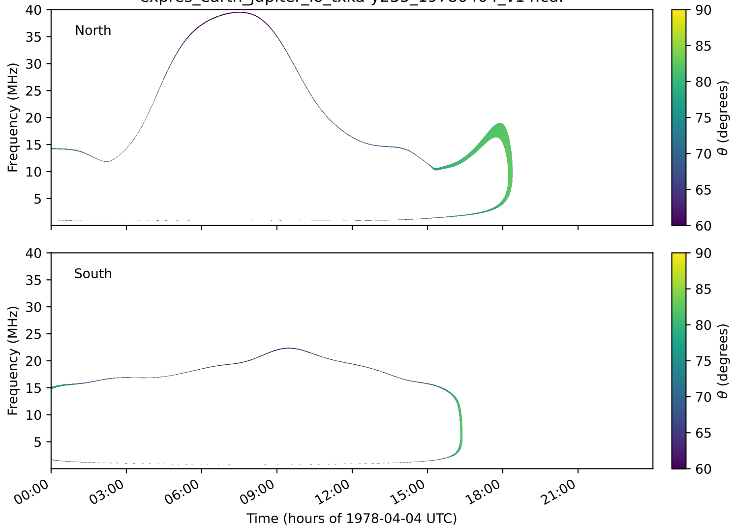
expres_earth_jupiter_io_txka-y235_19780404_v14.cdf
