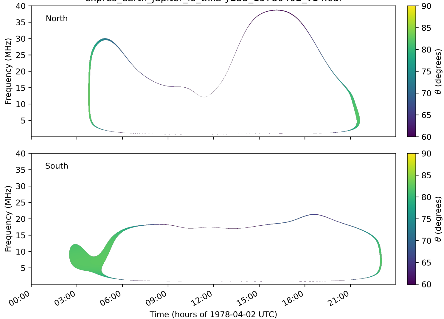
expres_earth_jupiter_io_txka-y235_19780402_v14.cdf
