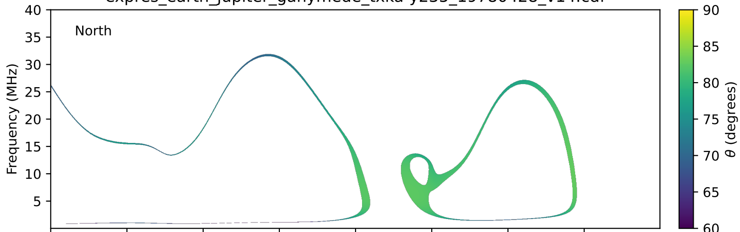
expres_earth_jupiter_ganymede_txka-y235_19780428_v14.cdf
