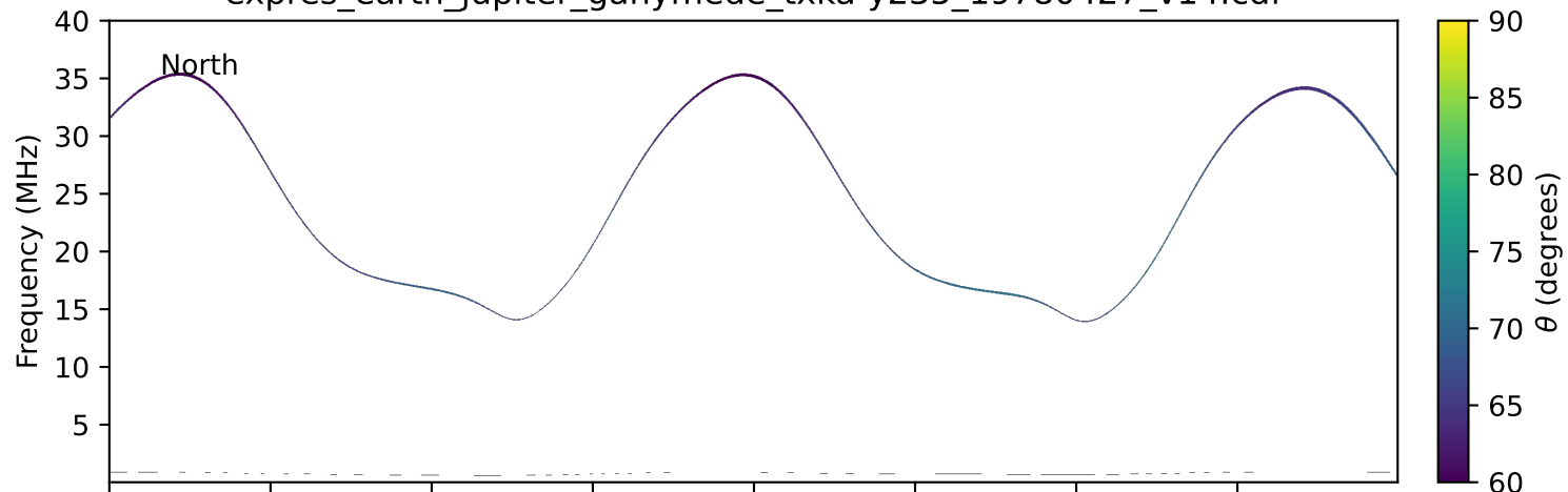
expres_earth_jupiter_ganymede_txka-y235_19780427_v14.cdf
