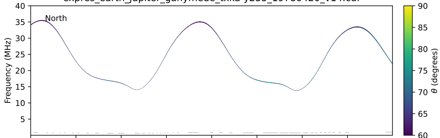
expres_earth_jupiter_ganymede_txka-y235_19780420_v14.cdf
