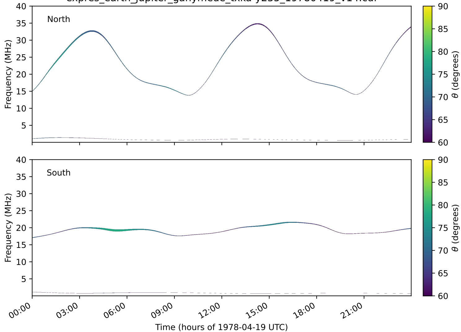
expres_earth_jupiter_ganymede_txka-y235_19780419_v14.cdf
