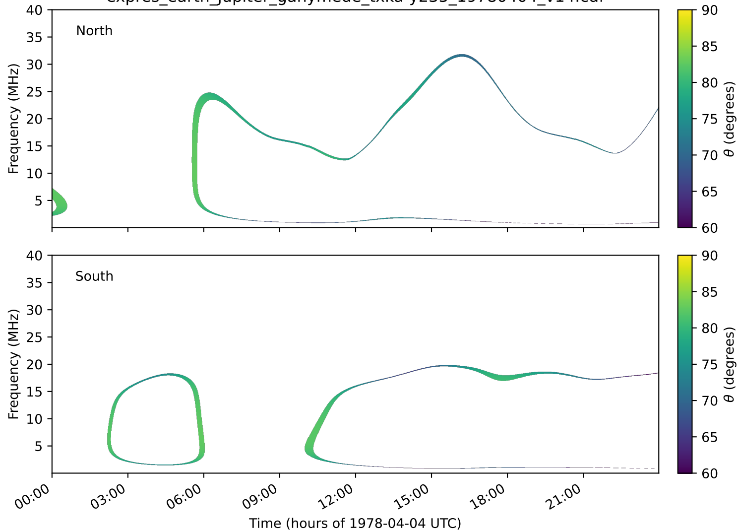
expres_earth_jupiter_ganymede_txka-y235_19780404_v14.cdf
