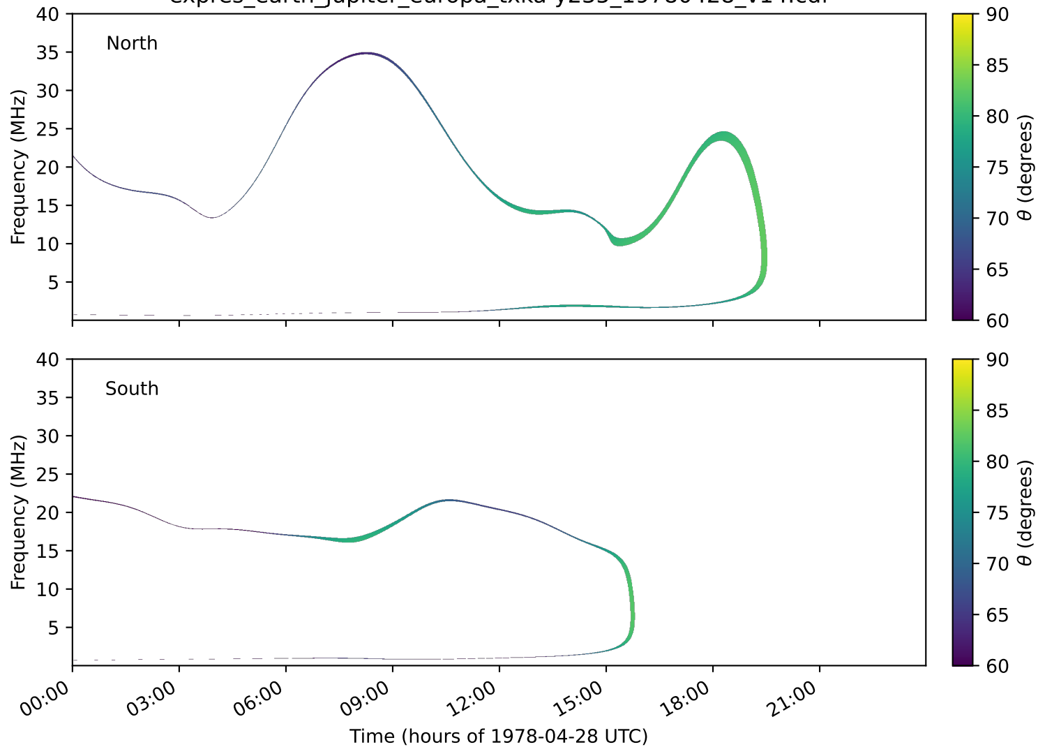
expres_earth_jupiter_europa_txka-y235_19780428_v14.cdf
