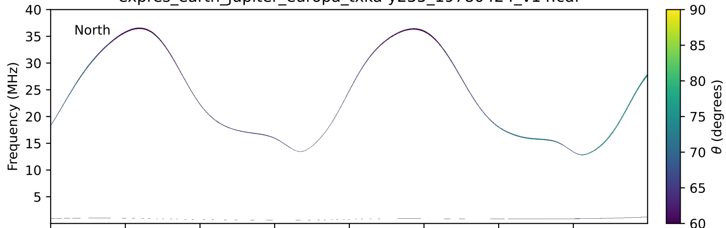
expres_earth_jupiter_europa_txka-y235_19780424_v14.cdf
