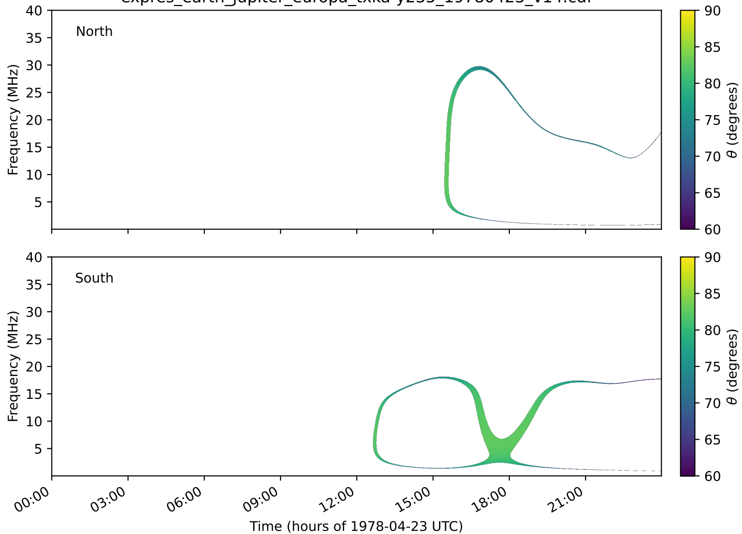
expres_earth_jupiter_europa_txka-y235_19780423_v14.cdf
