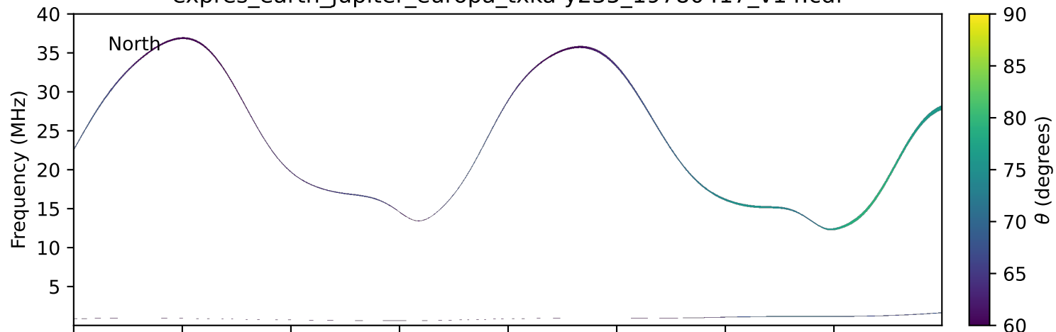
expres_earth_jupiter_europa_txka-y235_19780417_v14.cdf
