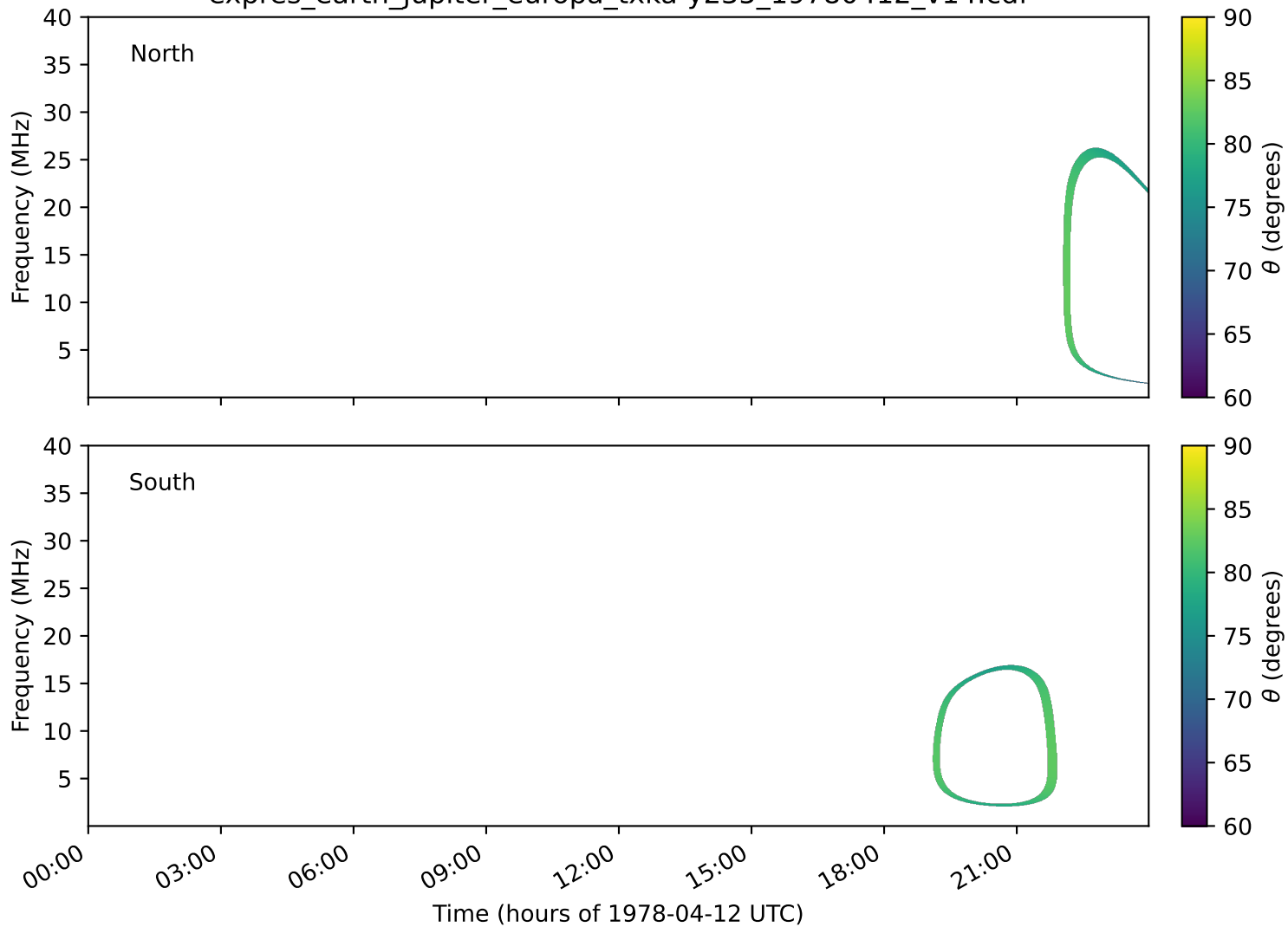
expres_earth_jupiter_europa_txka-y235_19780412_v14.cdf
