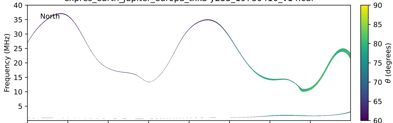
expres_earth_jupiter_europa_txka-y235_19780410_v14.cdf
