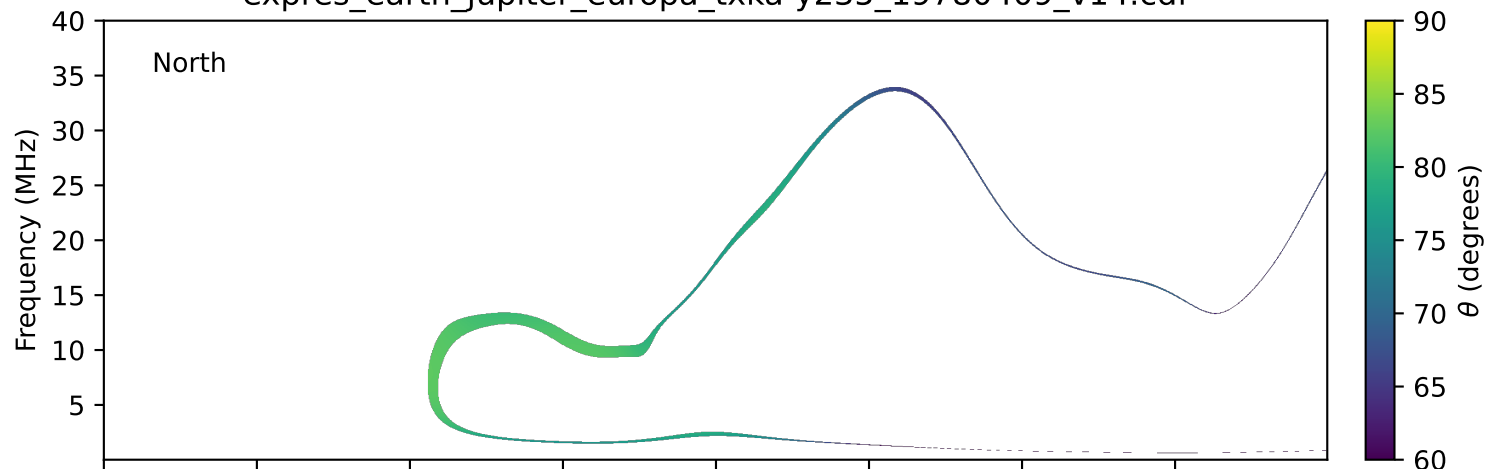
expres_earth_jupiter_europa_txka-y235_19780409_v14.cdf
