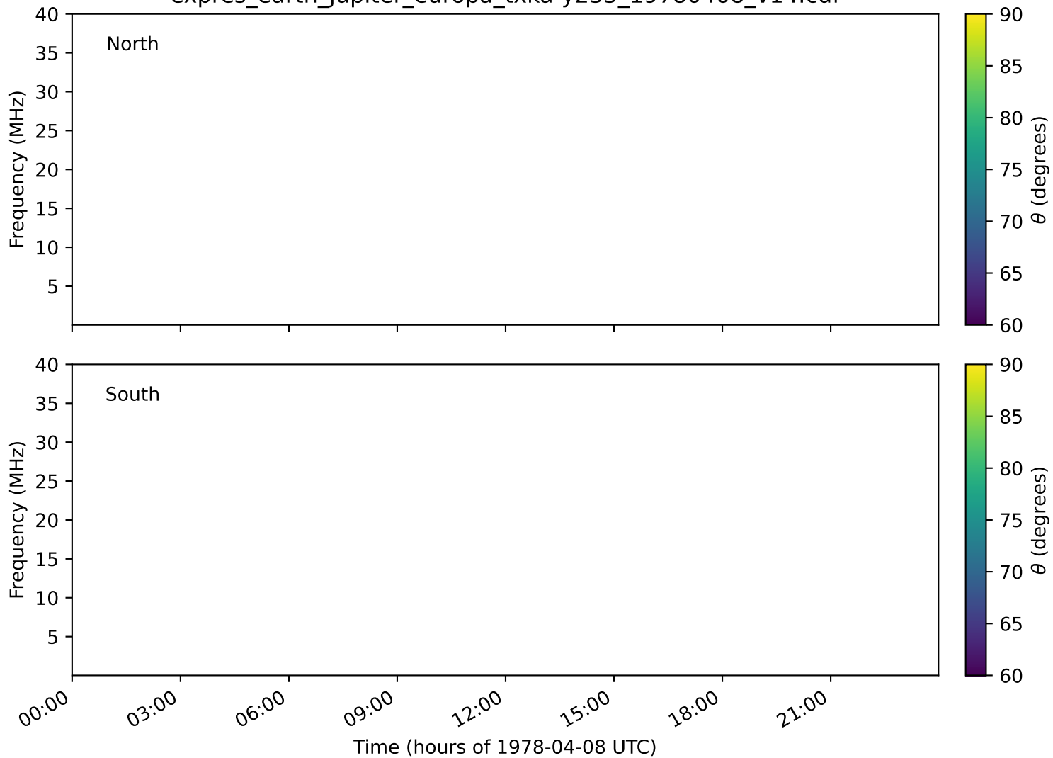
expres_earth_jupiter_europa_txka-y235_19780408_v14.cdf
