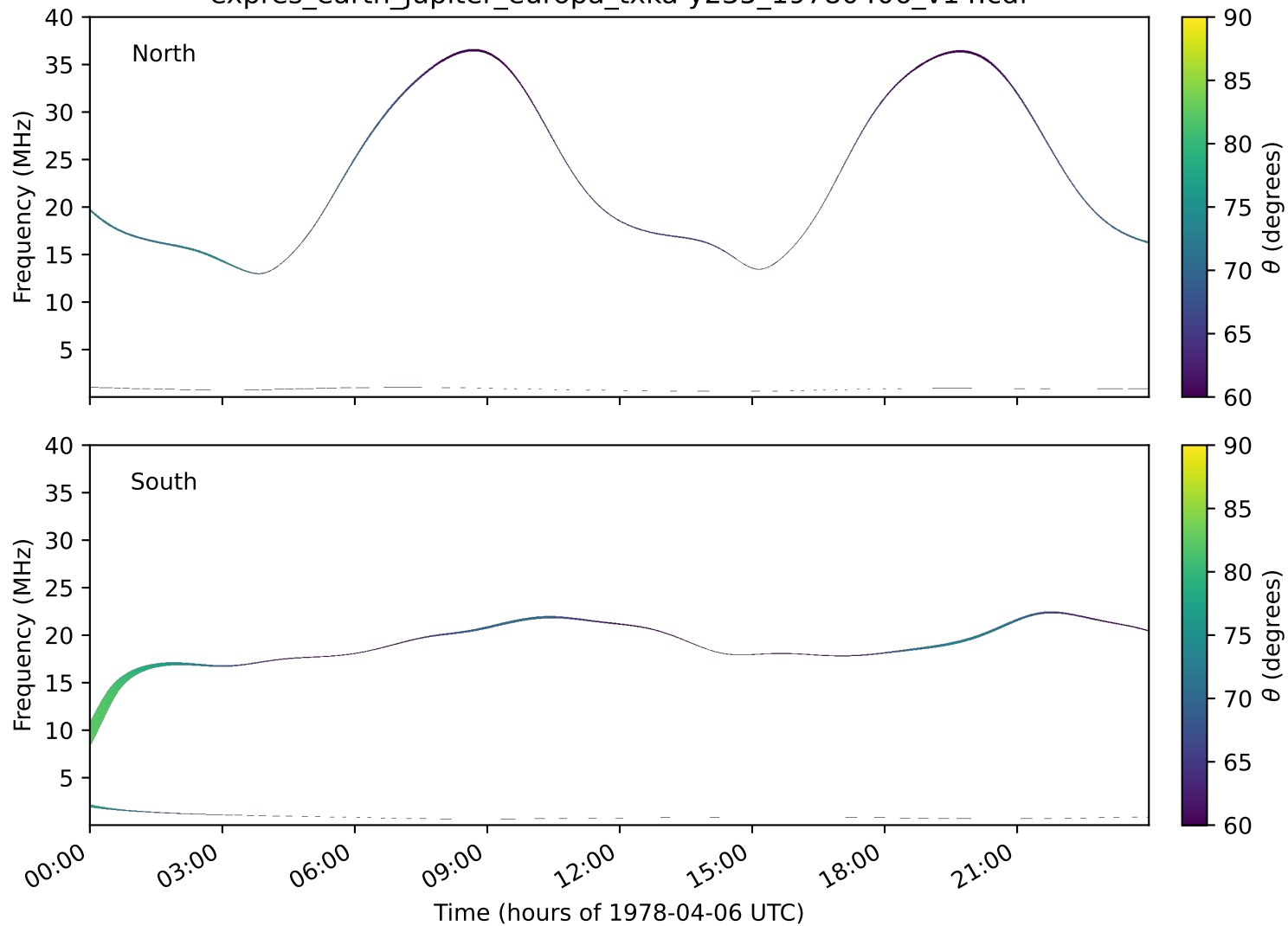
expres_earth_jupiter_europa_txka-y235_19780406_v14.cdf
