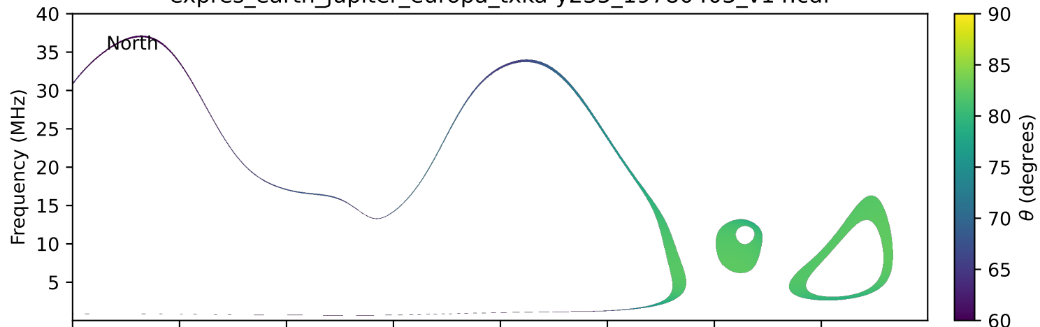
expres_earth_jupiter_europa_txka-y235_19780403_v14.cdf
