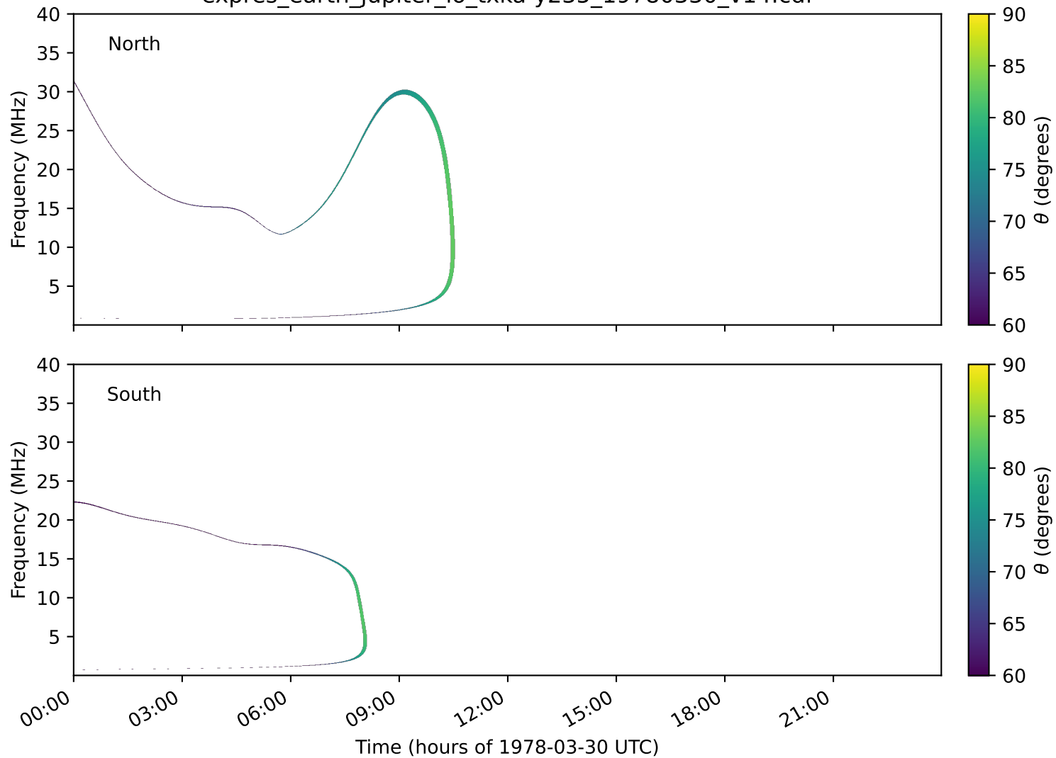
expres_earth_jupiter_io_txka-y235_19780330_v14.cdf
