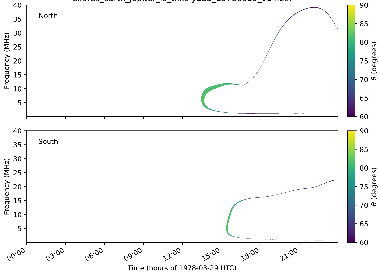
expres_earth_jupiter_io_txka-y235_19780329_v14.cdf
