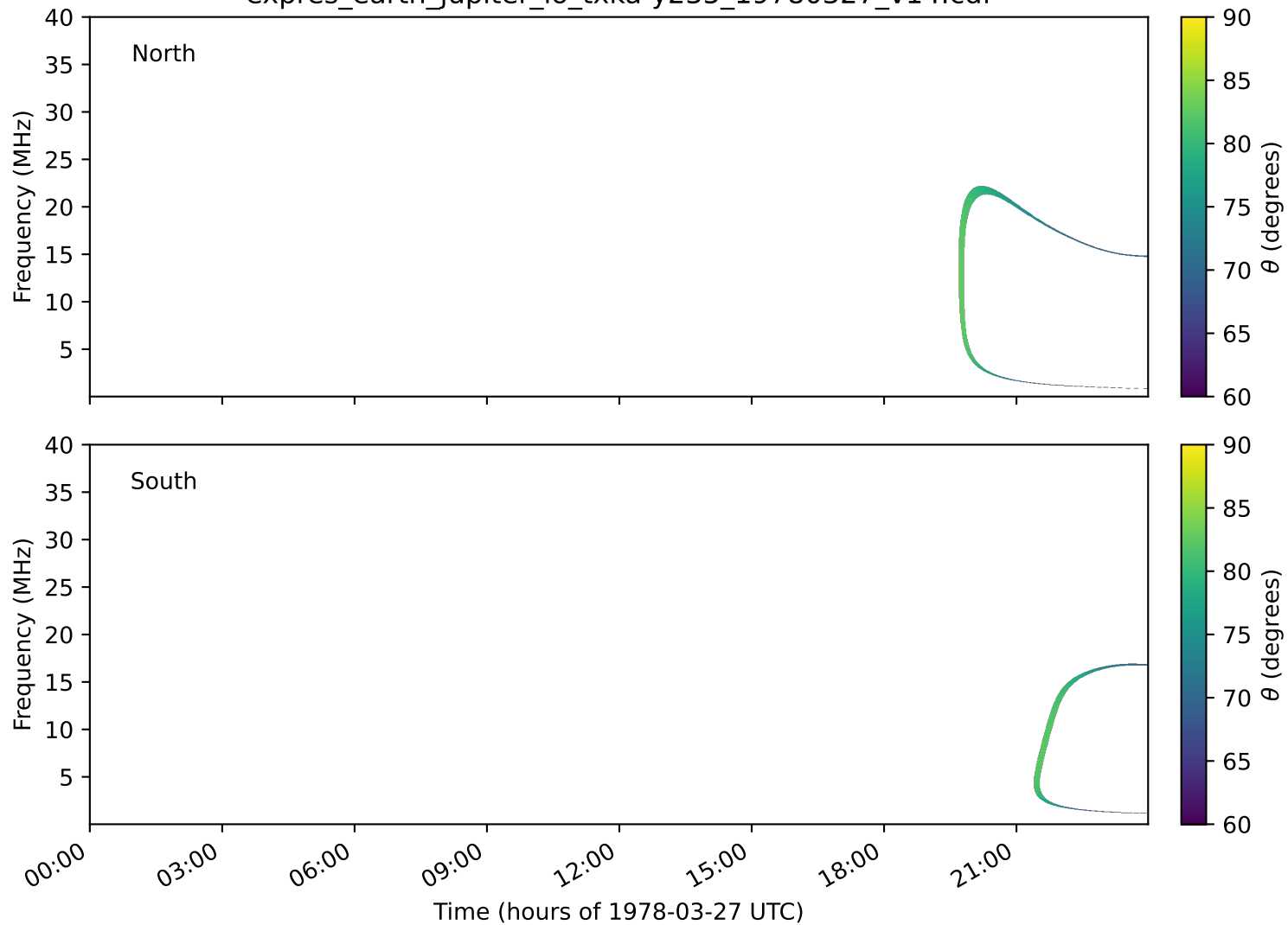
expres_earth_jupiter_io_txka-y235_19780327_v14.cdf
