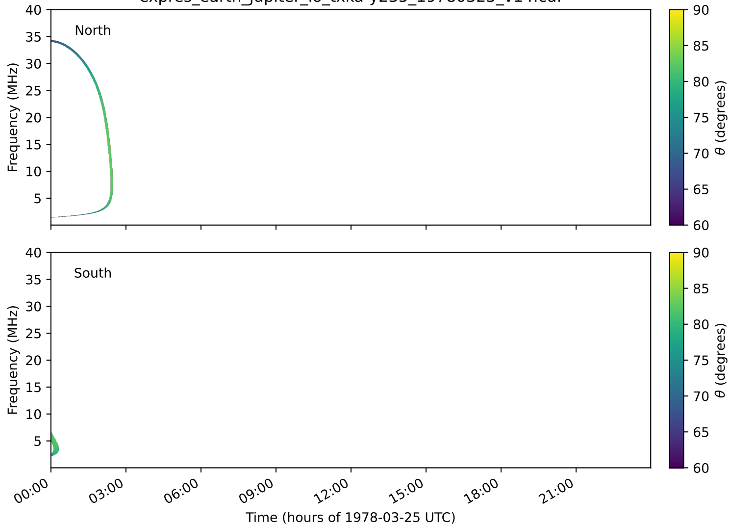
expres_earth_jupiter_io_txka-y235_19780325_v14.cdf
