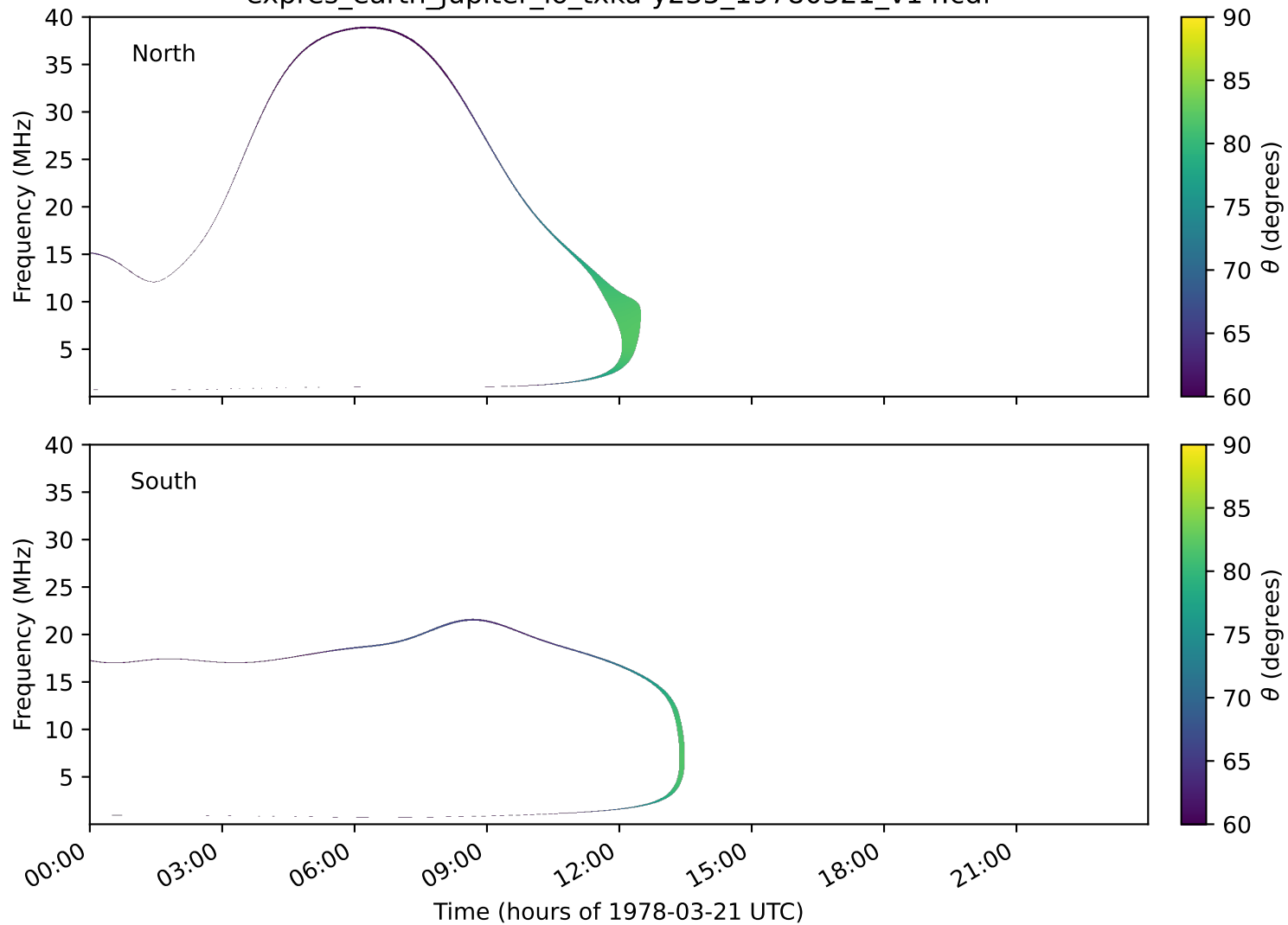
expres_earth_jupiter_io_txka-y235_19780321_v14.cdf
