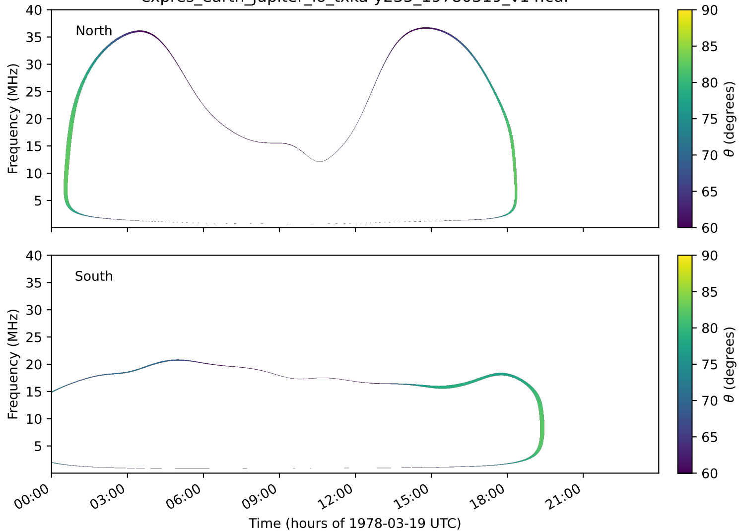
expres_earth_jupiter_io_txka-y235_19780319_v14.cdf
