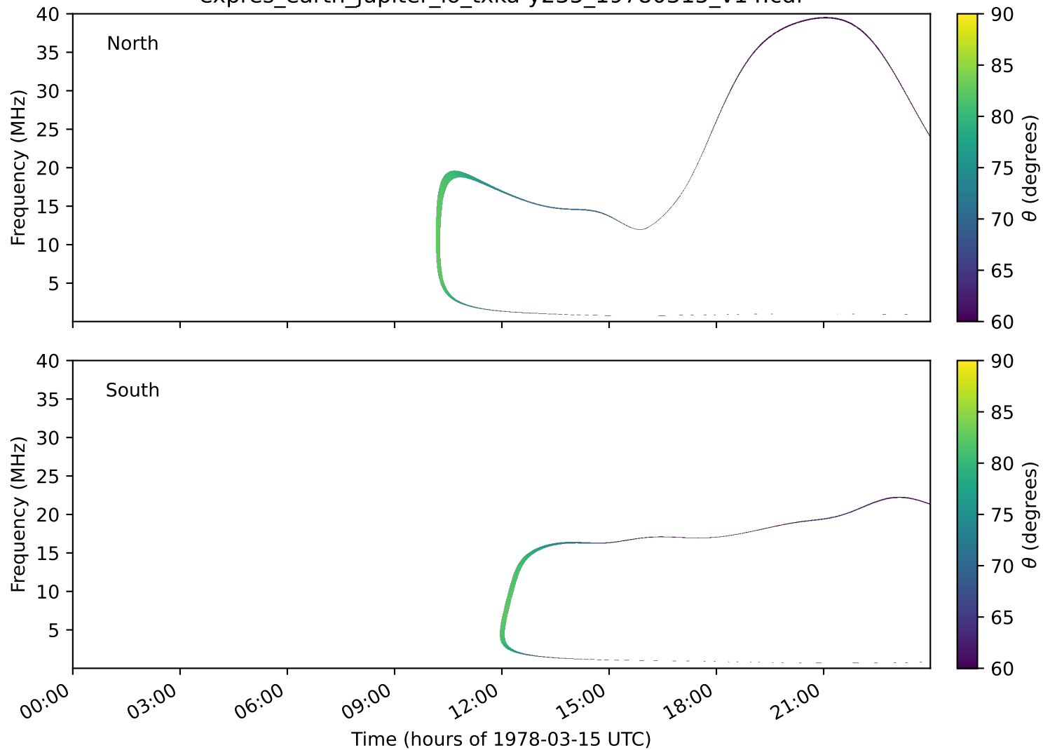
expres_earth_jupiter_io_txka-y235_19780315_v14.cdf
