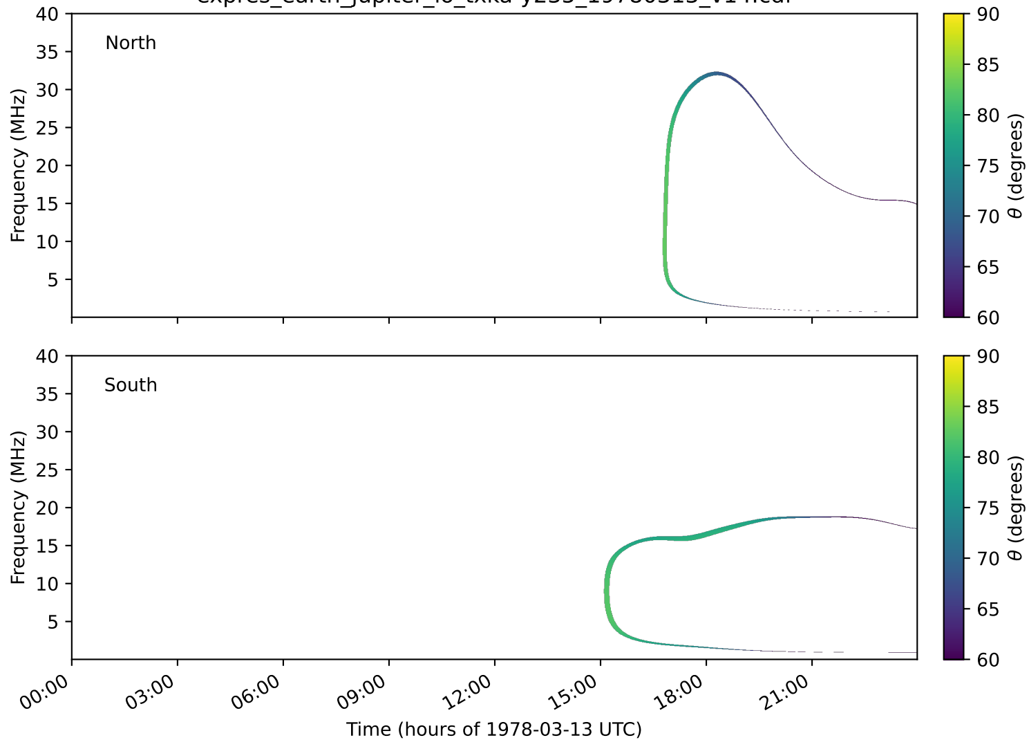
expres_earth_jupiter_io_txka-y235_19780313_v14.cdf
