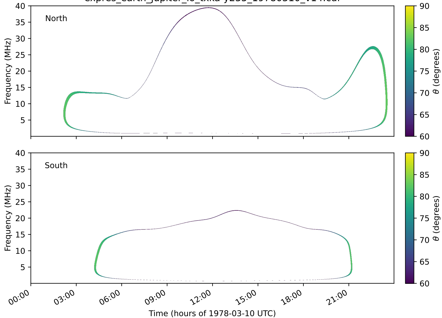
expres_earth_jupiter_io_txka-y235_19780310_v14.cdf
