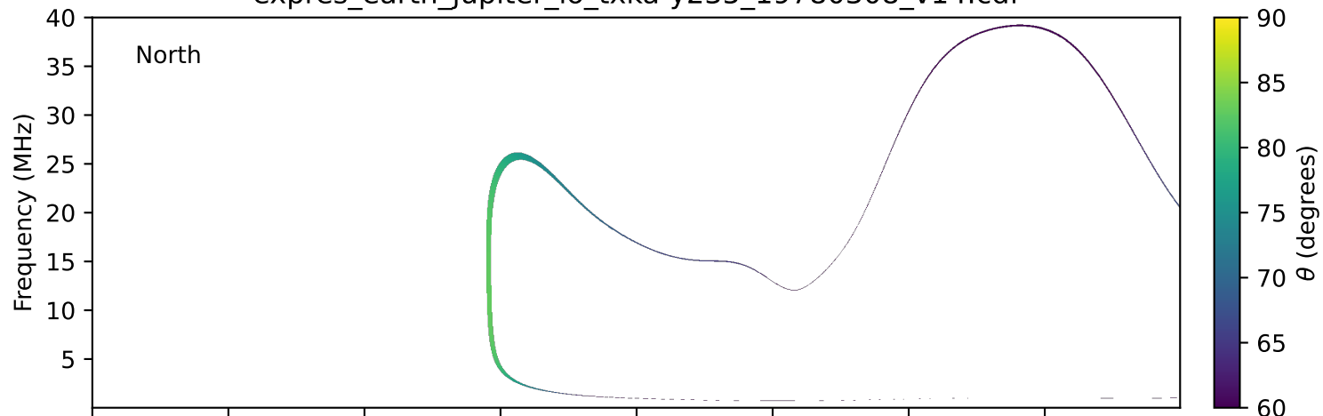
expres_earth_jupiter_io_txka-y235_19780308_v14.cdf
