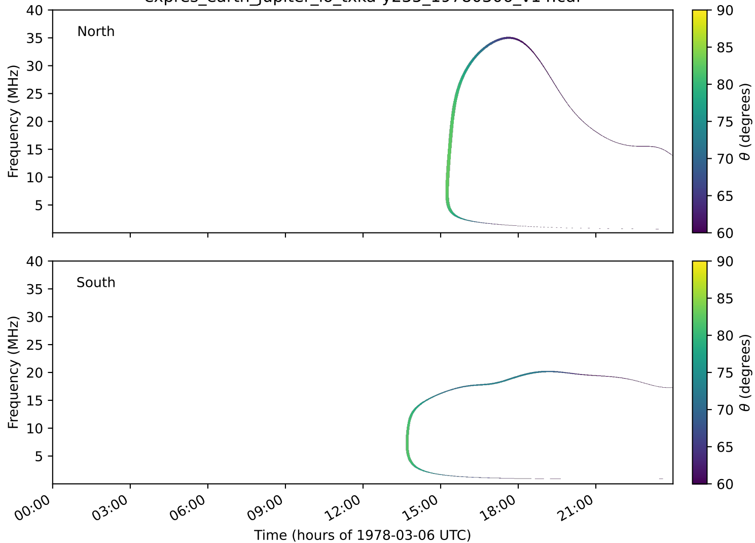
expres_earth_jupiter_io_txka-y235_19780306_v14.cdf
