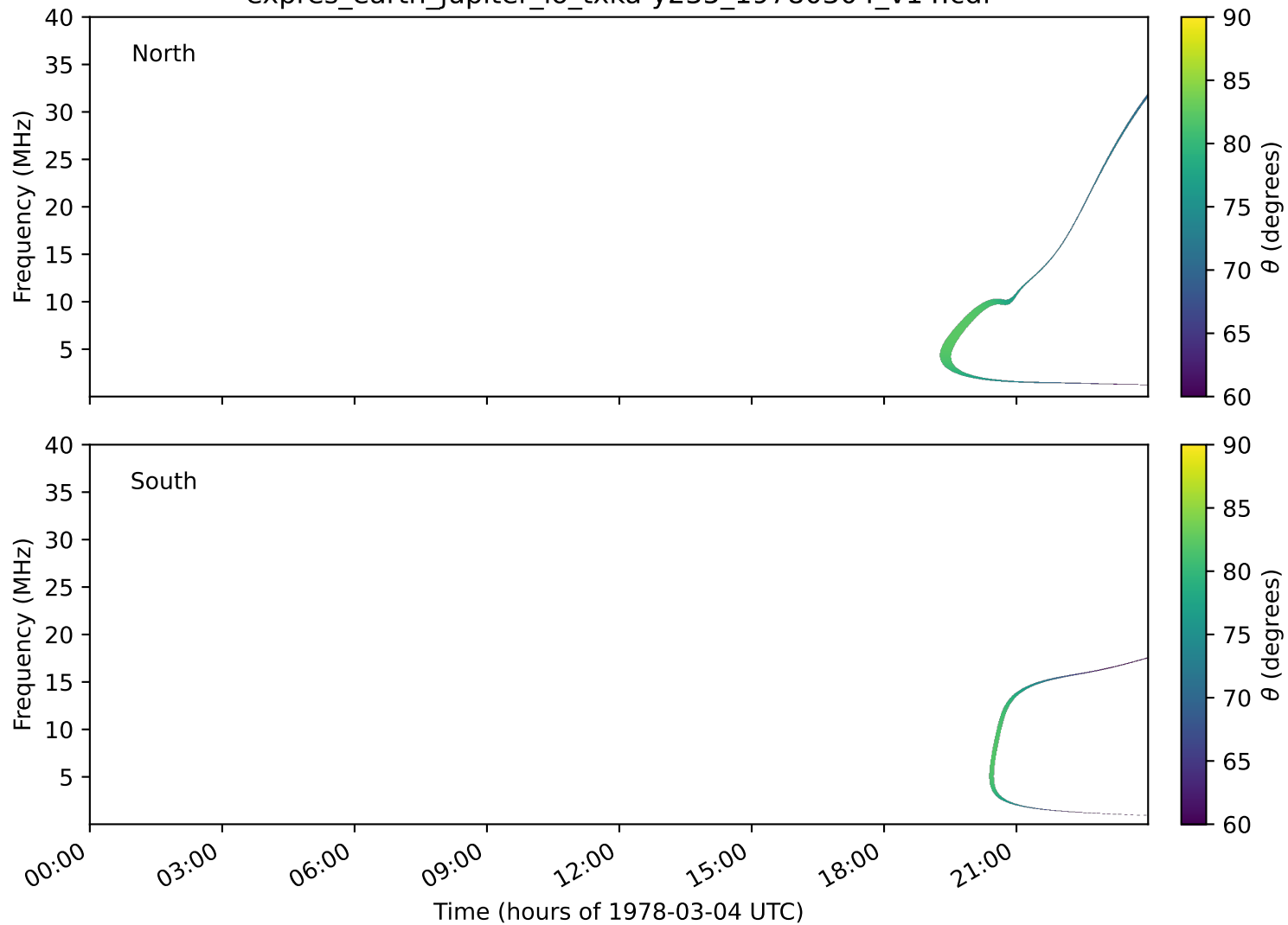
expres_earth_jupiter_io_txka-y235_19780304_v14.cdf
