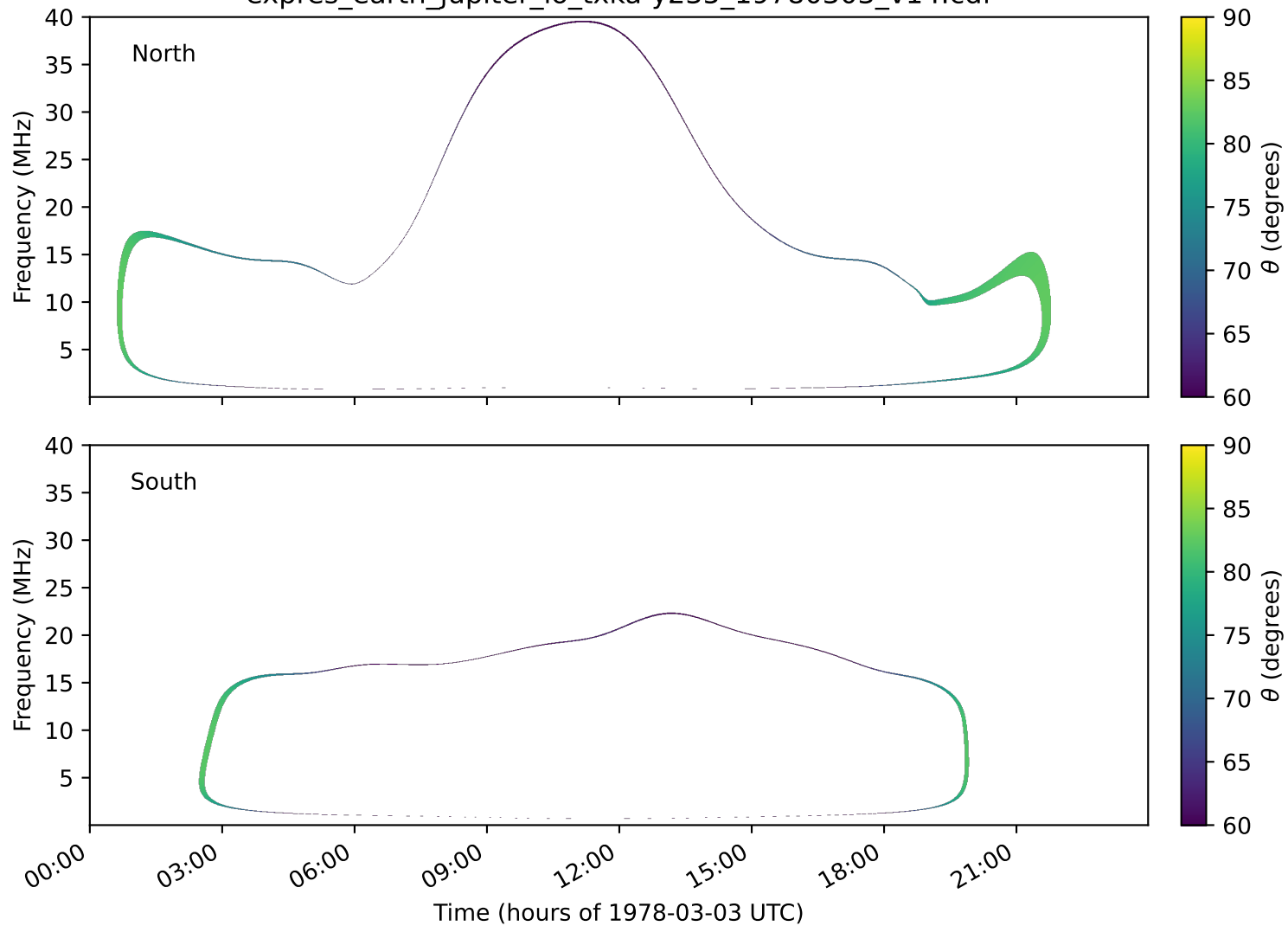
expres_earth_jupiter_io_txka-y235_19780303_v14.cdf
