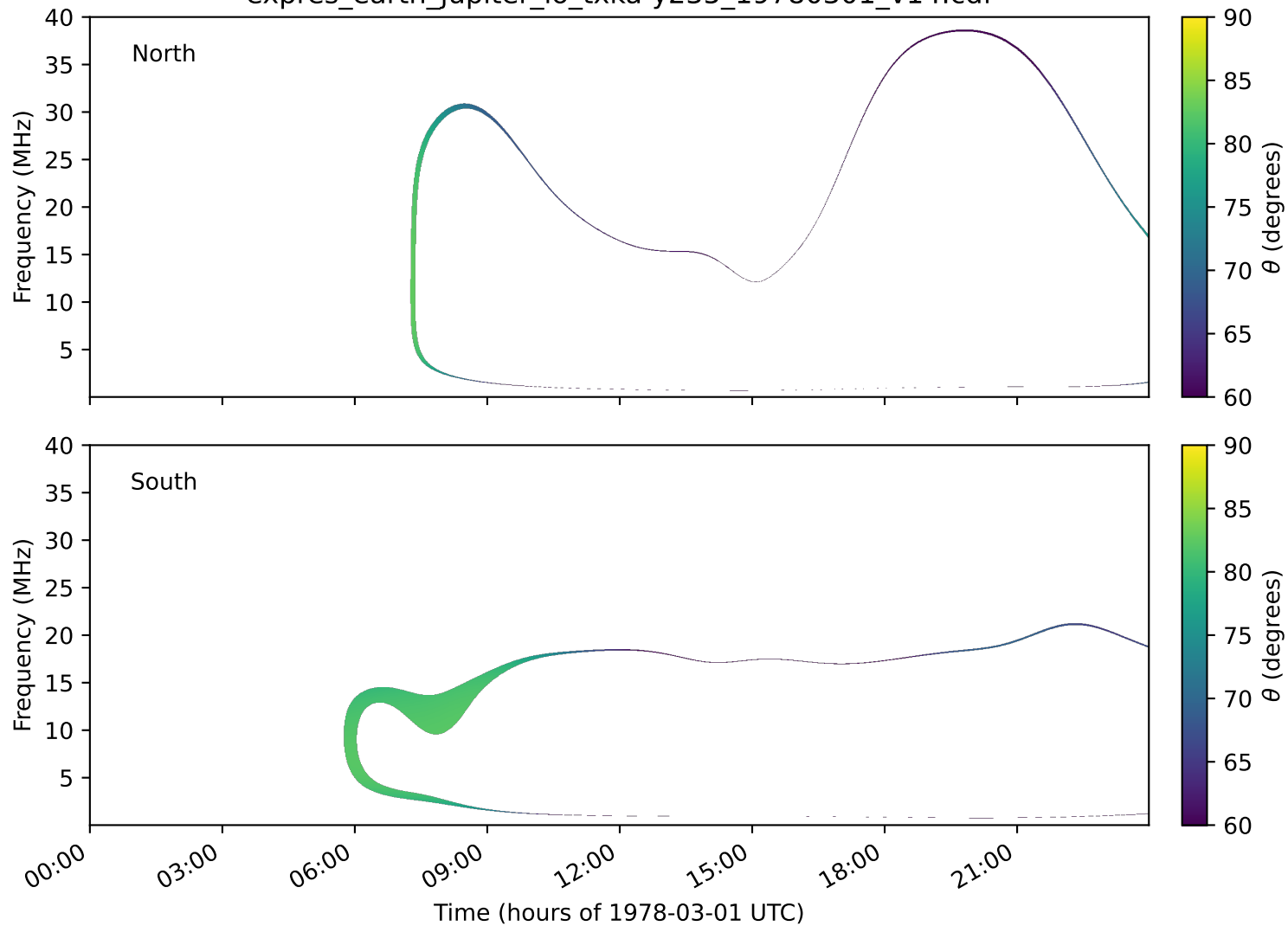
expres_earth_jupiter_io_txka-y235_19780301_v14.cdf
