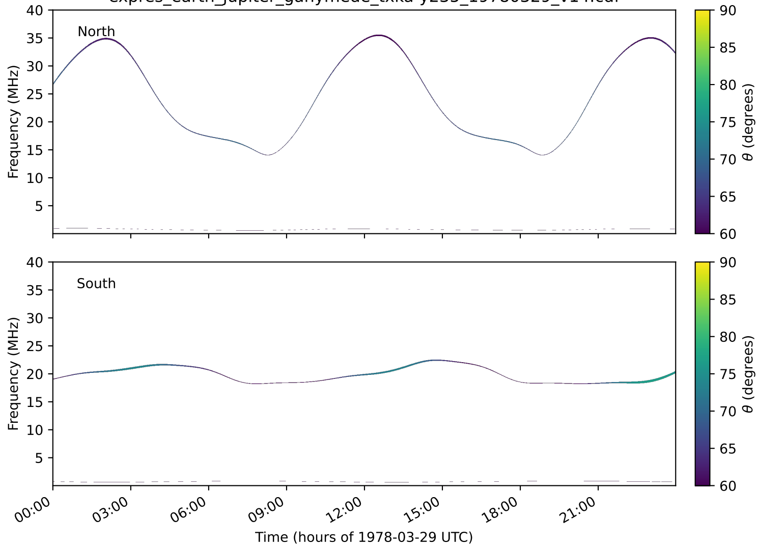
expres_earth_jupiter_ganymede_txka-y235_19780329_v14.cdf
