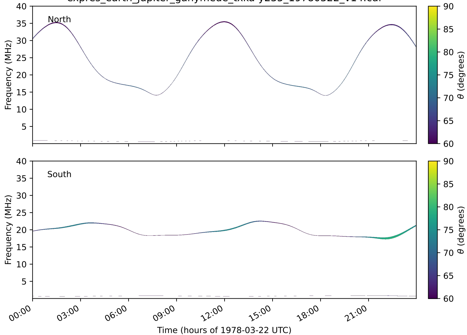
expres_earth_jupiter_ganymede_txka-y235_19780322_v14.cdf
