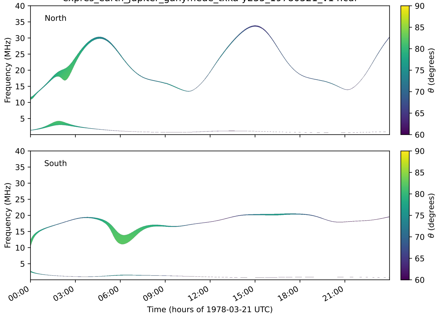
expres_earth_jupiter_ganymede_txka-y235_19780321_v14.cdf
