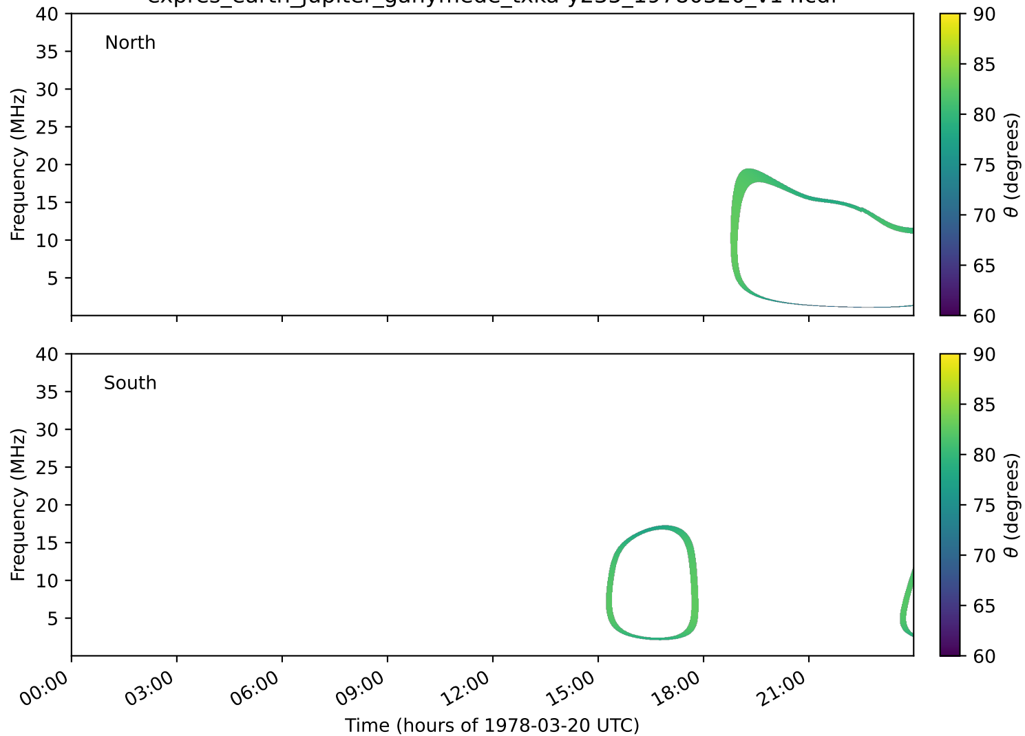
expres_earth_jupiter_ganymede_txka-y235_19780320_v14.cdf
