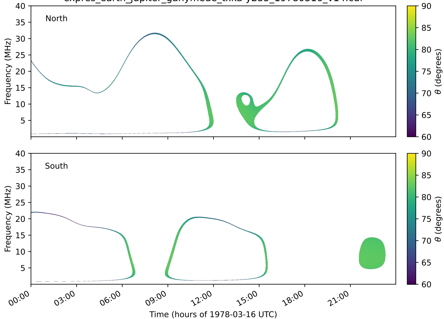
expres_earth_jupiter_ganymede_txka-y235_19780316_v14.cdf
