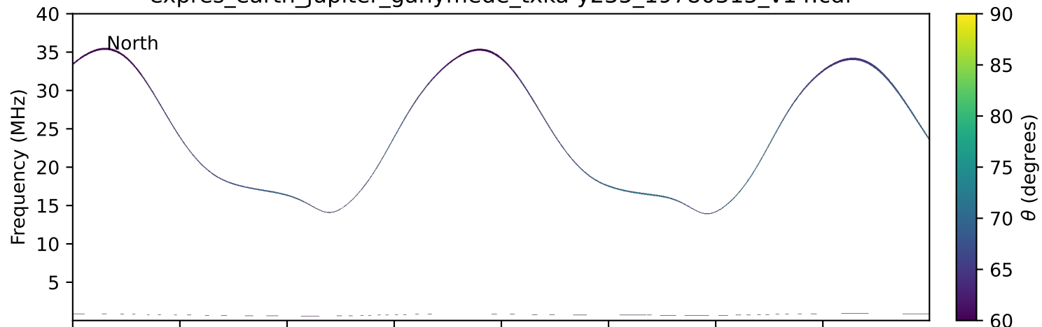
expres_earth_jupiter_ganymede_txka-y235_19780315_v14.cdf
