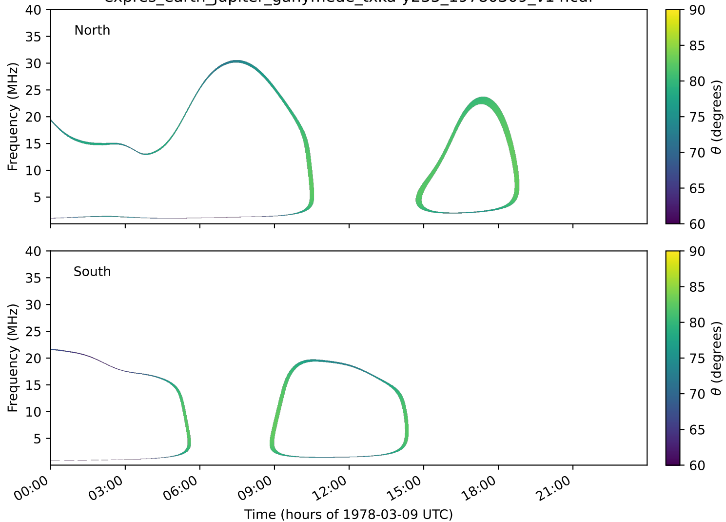
expres_earth_jupiter_ganymede_txka-y235_19780309_v14.cdf
