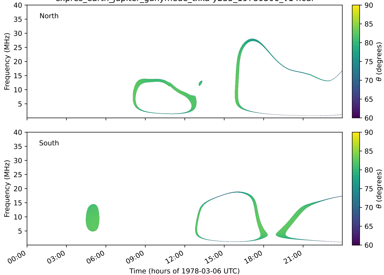
expres_earth_jupiter_ganymede_txka-y235_19780306_v14.cdf
