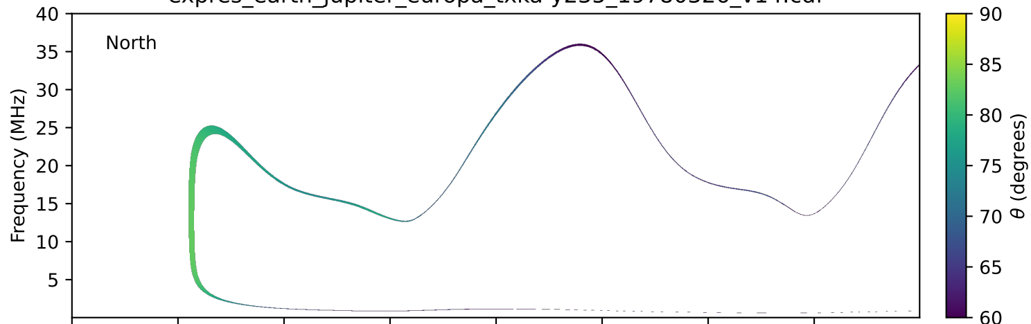
expres_earth_jupiter_europa_txka-y235_19780326_v14.cdf
