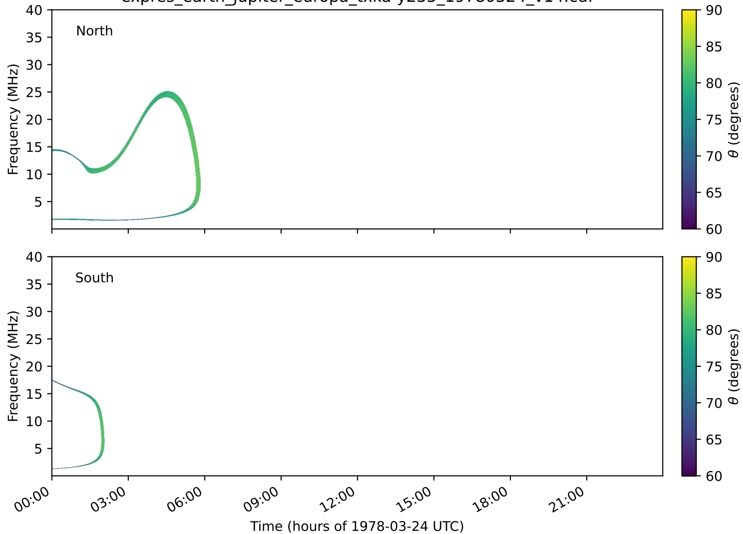
expres_earth_jupiter_europa_txka-y235_19780324_v14.cdf
