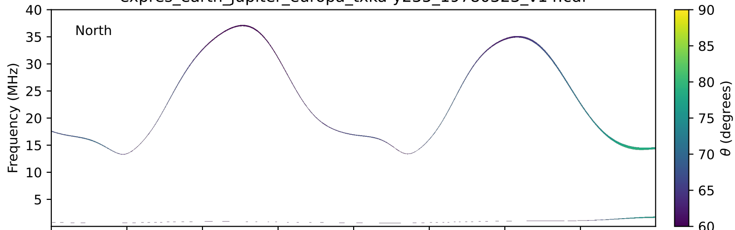
expres_earth_jupiter_europa_txka-y235_19780323_v14.cdf
