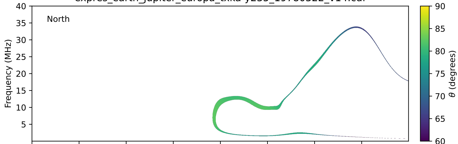
expres_earth_jupiter_europa_txka-y235_19780322_v14.cdf
