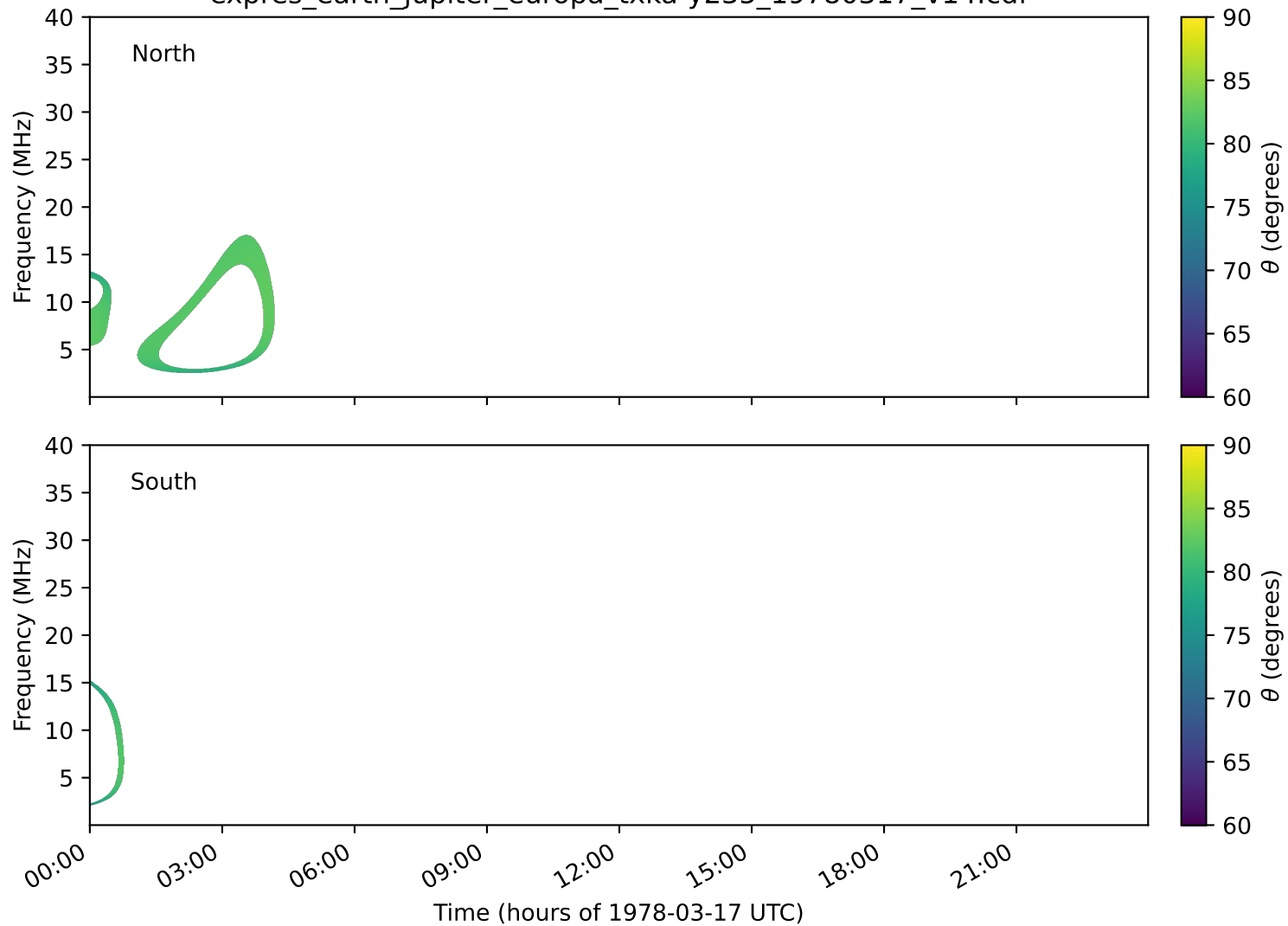
expres_earth_jupiter_europa_txka-y235_19780317_v14.cdf
