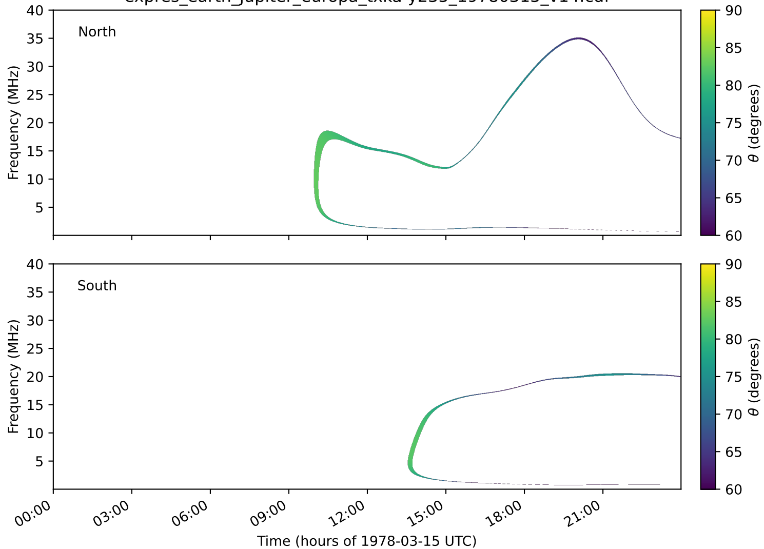
expres_earth_jupiter_europa_txka-y235_19780315_v14.cdf
