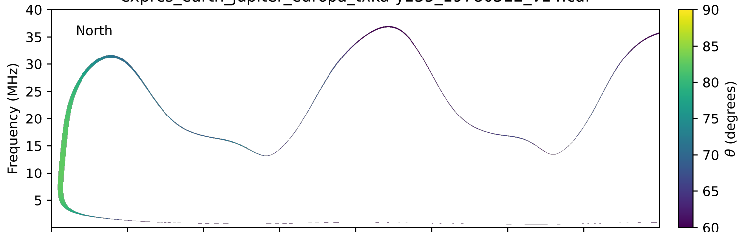
expres_earth_jupiter_europa_txka-y235_19780312_v14.cdf
