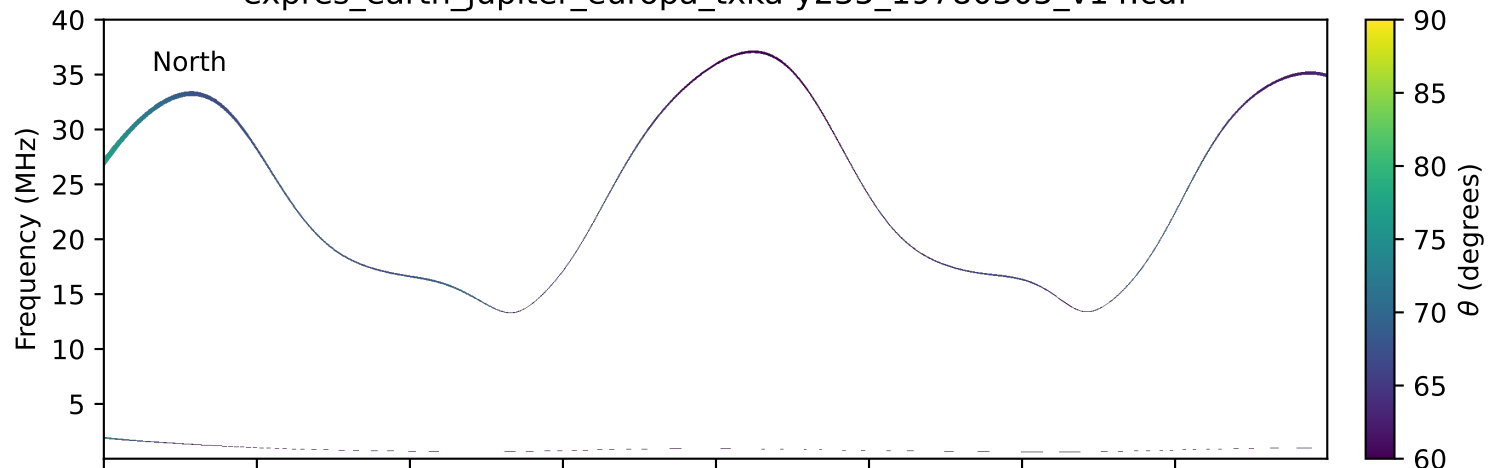
expres_earth_jupiter_europa_txka-y235_19780305_v14.cdf
